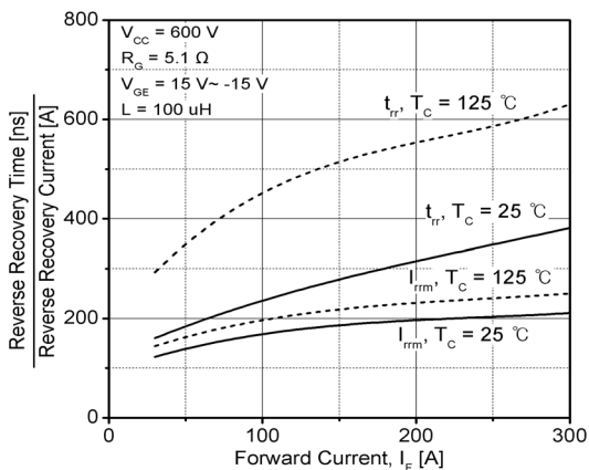
Fig 11. Typical Recovery Characteristics of Diode
